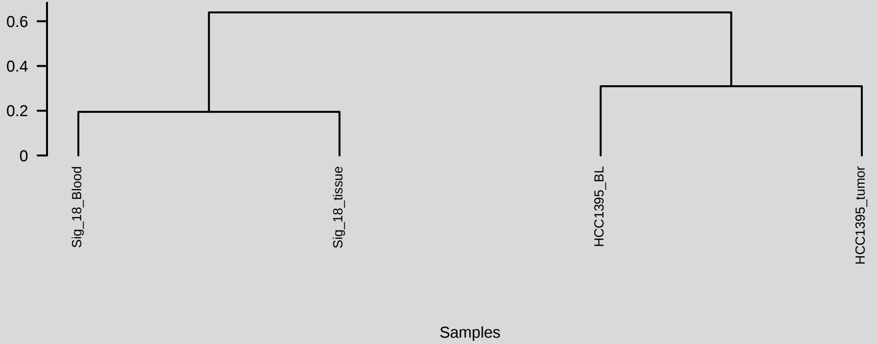
Cluster Dendrogram
